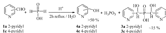
Scheme 3. Reaction of hypophosphorous acid with 2-pyridine- and 4-pyridinecarboxaldehyde in the presence of HCl.
