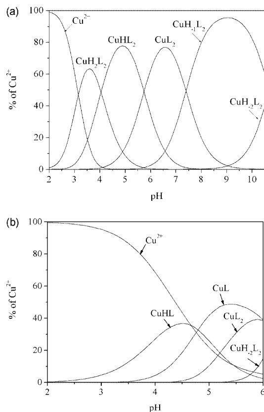
Figure 2. Species distribution curves for (a) Cu II -L 3 and (b) Cu II -L 4 as a function of pH.
